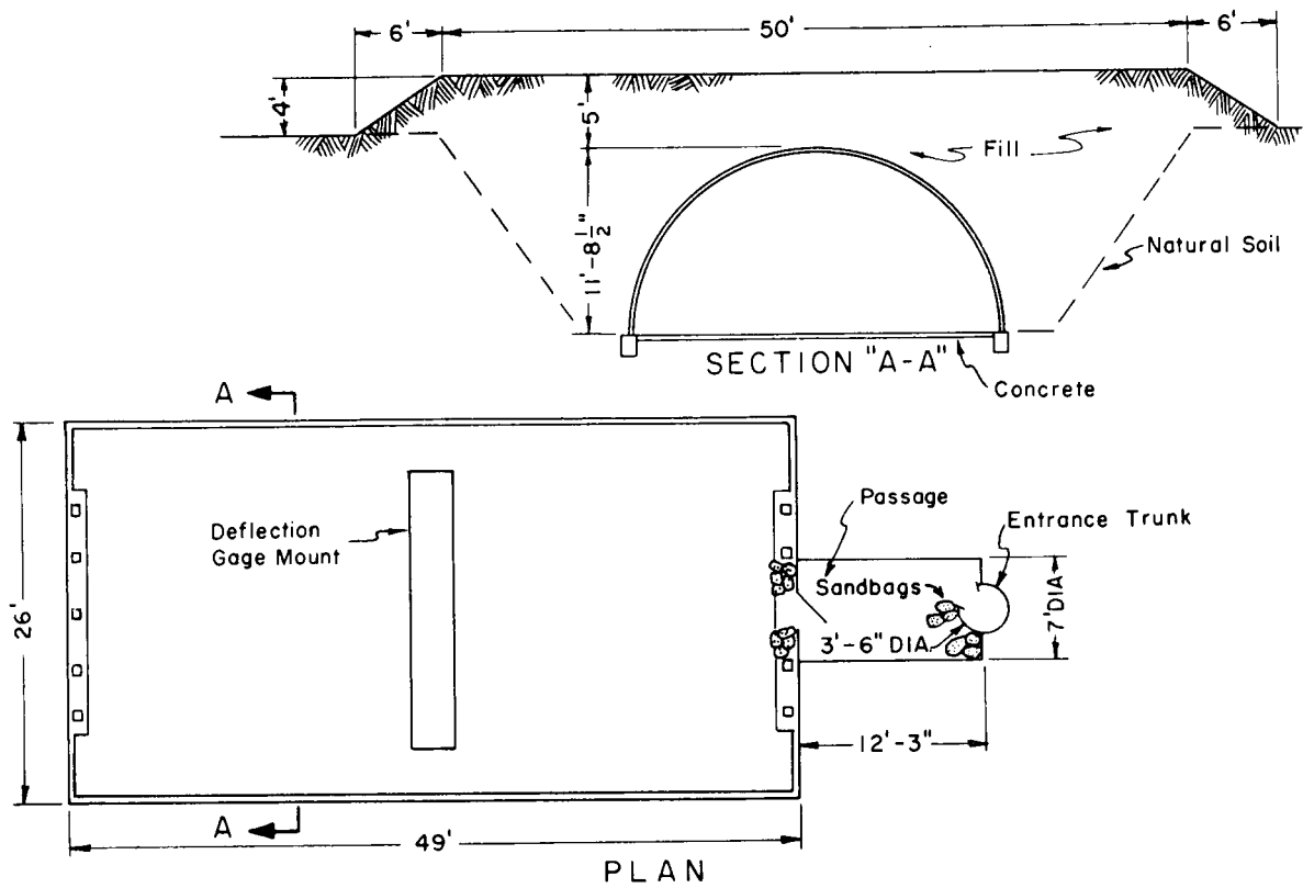
Fig. 4—Plan and section of structure 3.3b.
